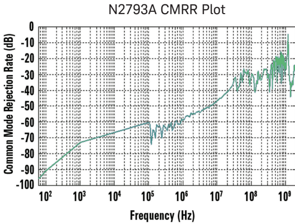
Figure 12. Frequency response ( V_{out}/V_{in} ) of N2793A/N2819A when inputs driven in common (Common Mode Rejection)
